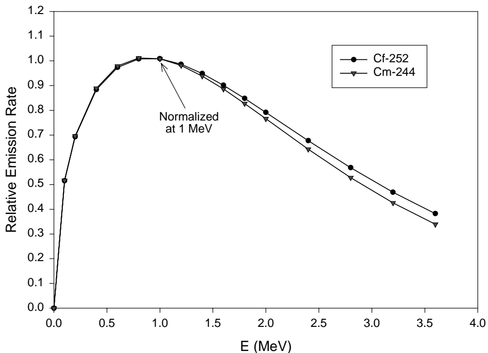
Fig. A-1. Neutron energy spectra for ^{252}\text{Cf} and ^{244}\text{Cm} are shown, normalized to the same emission rate at 1 MeV. The ^{252}\text{Cf} spectrum is slightly “harder” than that of ^{244}\text{Cm} . These are Watt spectra, using parameters from the MCNP manual.
